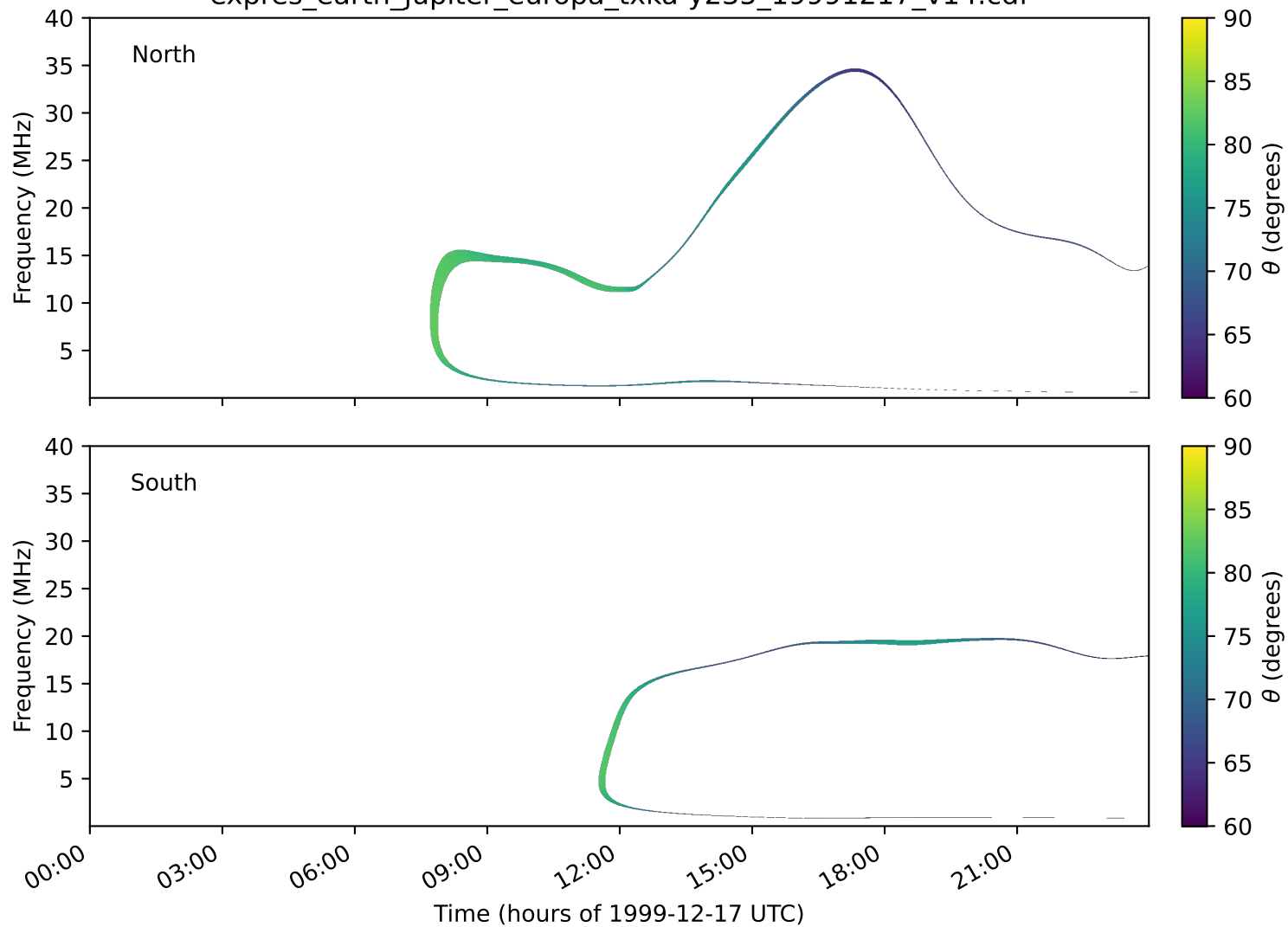
expres_earth_jupiter_europa_txka-y235_19991217_v14.cdf
