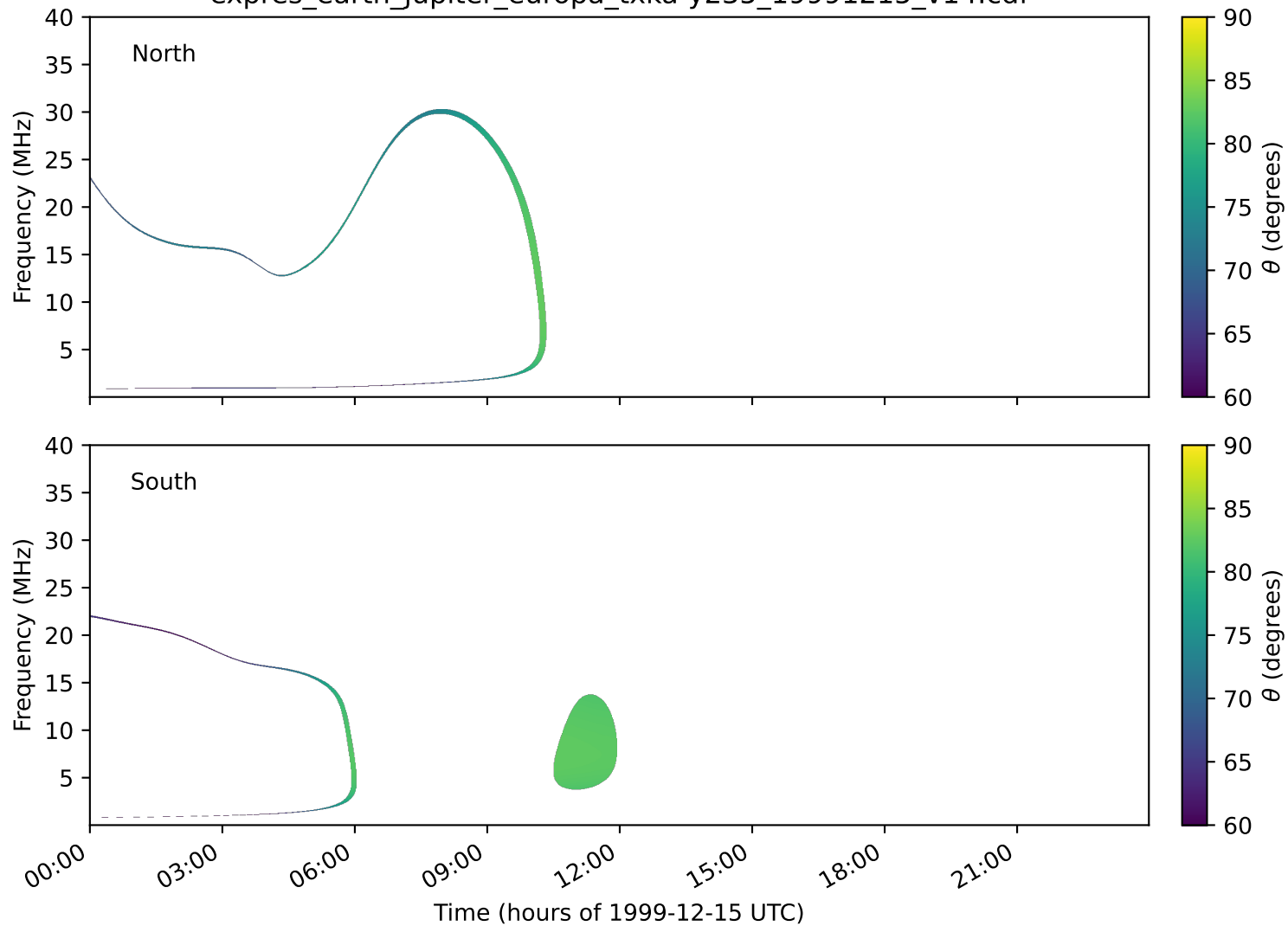
expres_earth_jupiter_europa_txka-y235_19991215_v14.cdf
