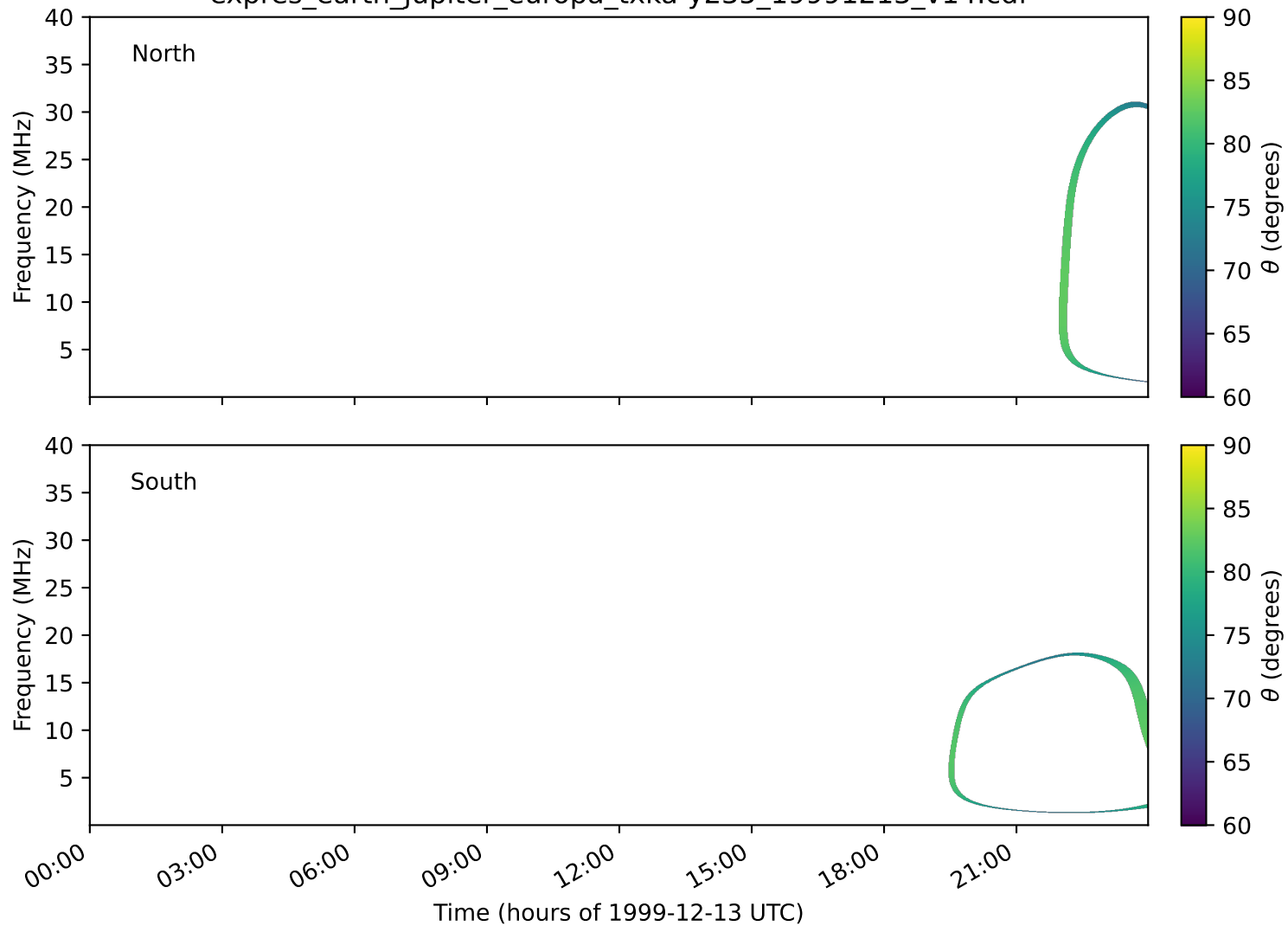
expres_earth_jupiter_europa_txka-y235_19991213_v14.cdf
