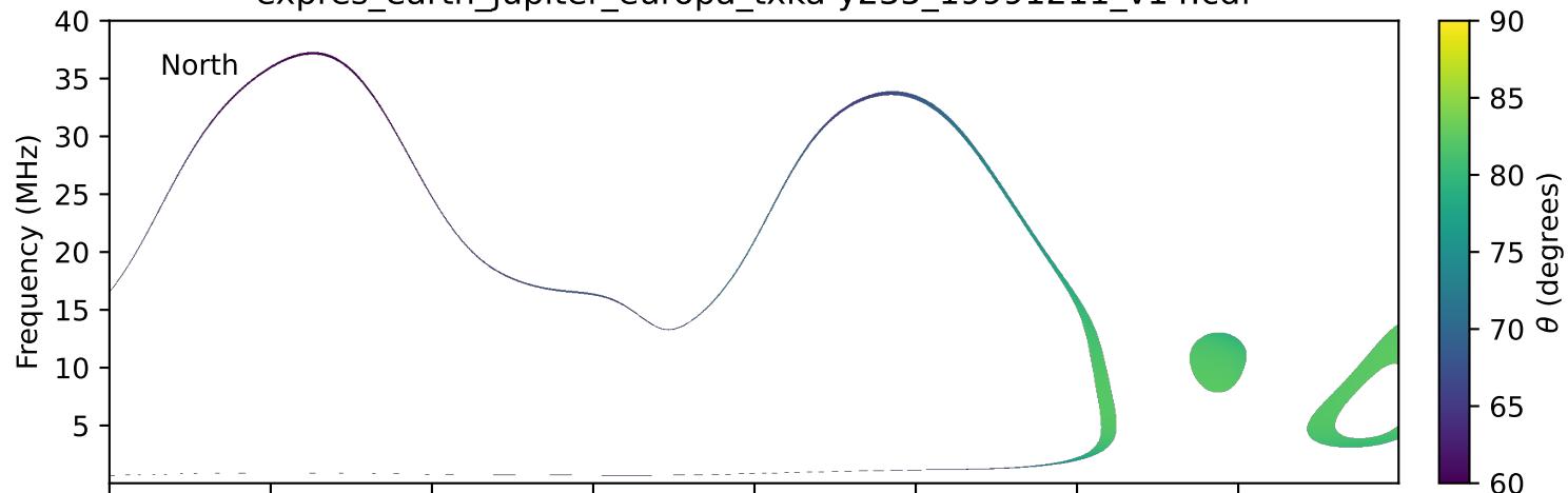
expres_earth_jupiter_europa_txka-y235_19991211_v14.cdf
