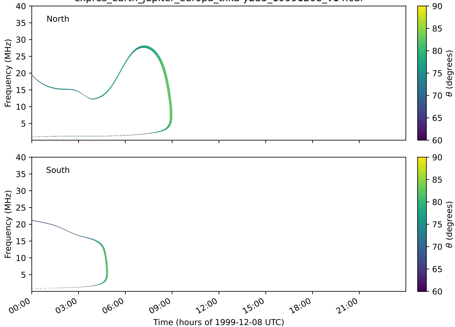
expres_earth_jupiter_europa_txka-y235_19991208_v14.cdf
