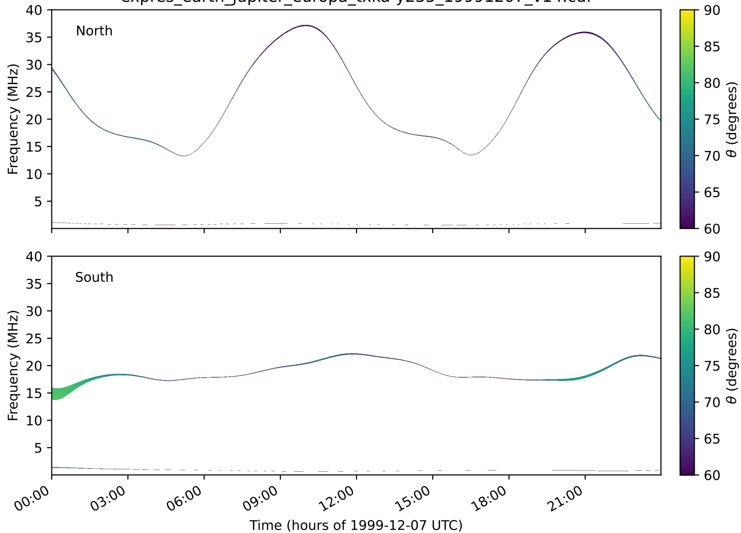
expres_earth_jupiter_europa_txka-y235_19991207_v14.cdf
