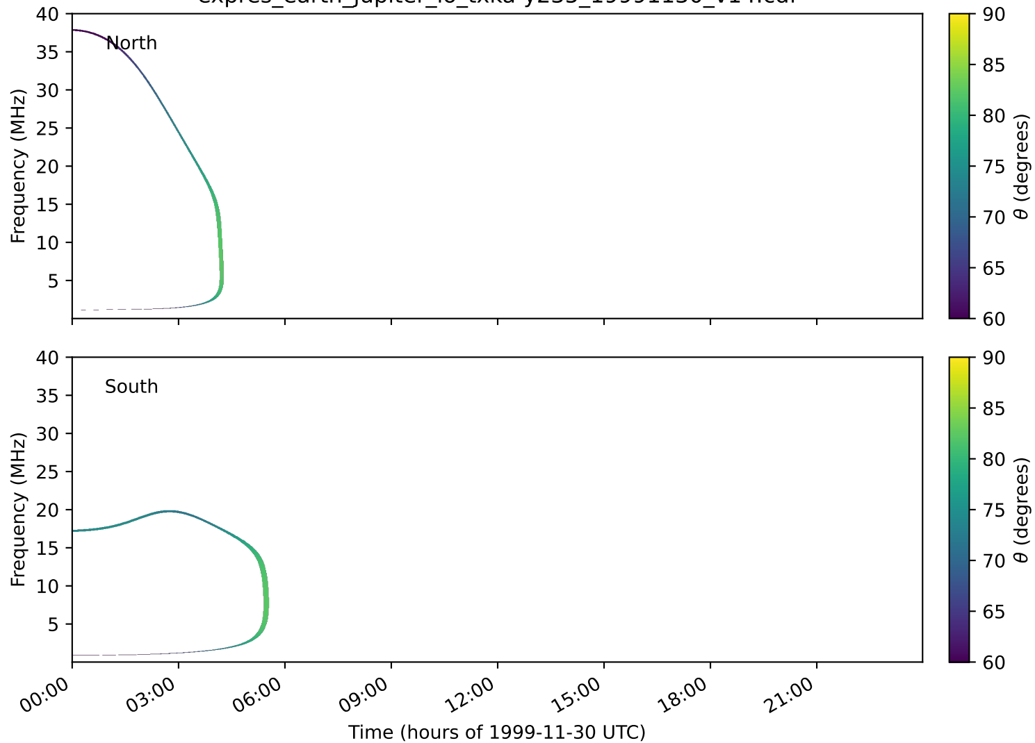
expres_earth_jupiter_io_txka-y235_19991130_v14.cdf
