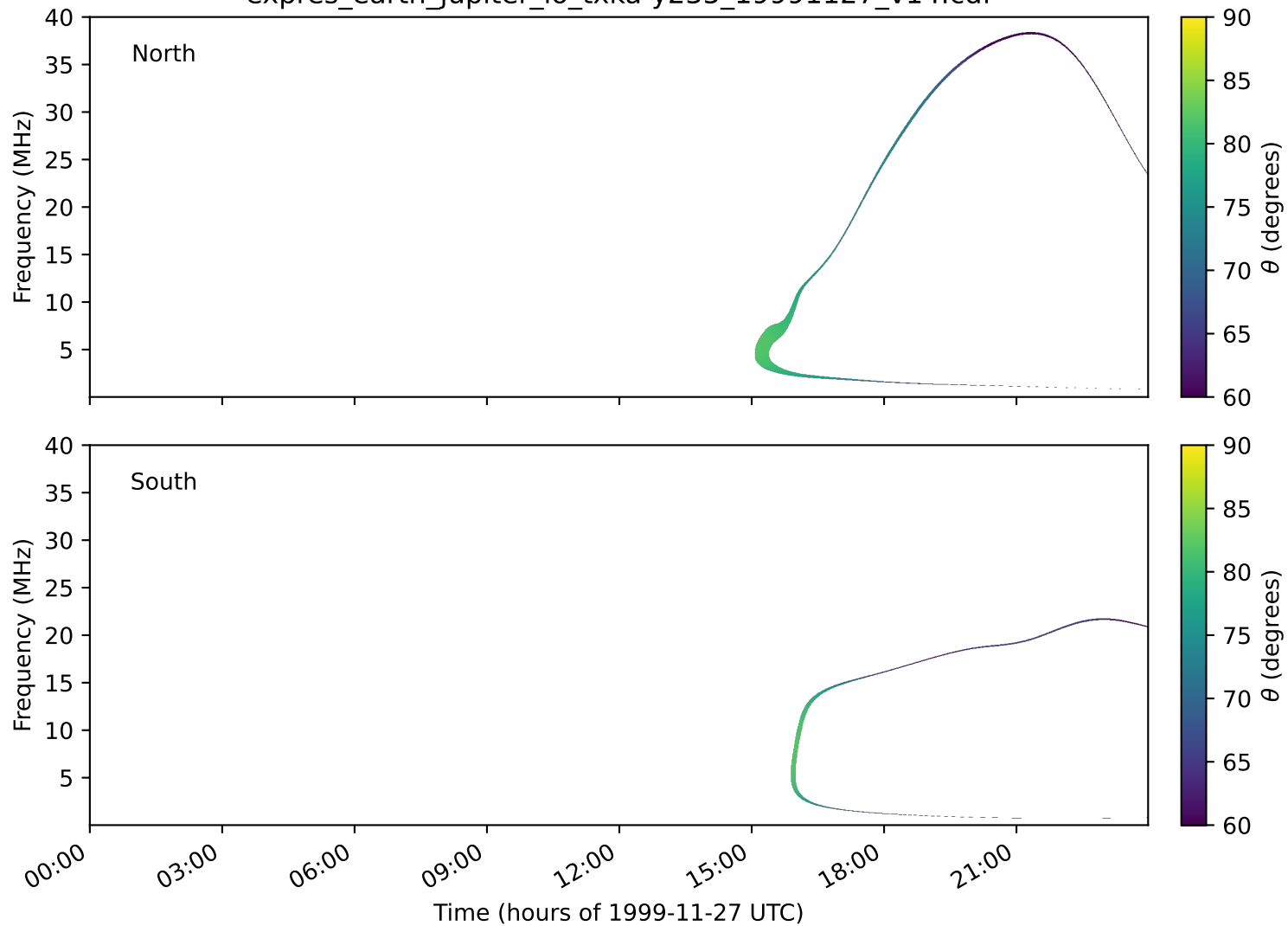
expres_earth_jupiter_io_txka-y235_19991127_v14.cdf
