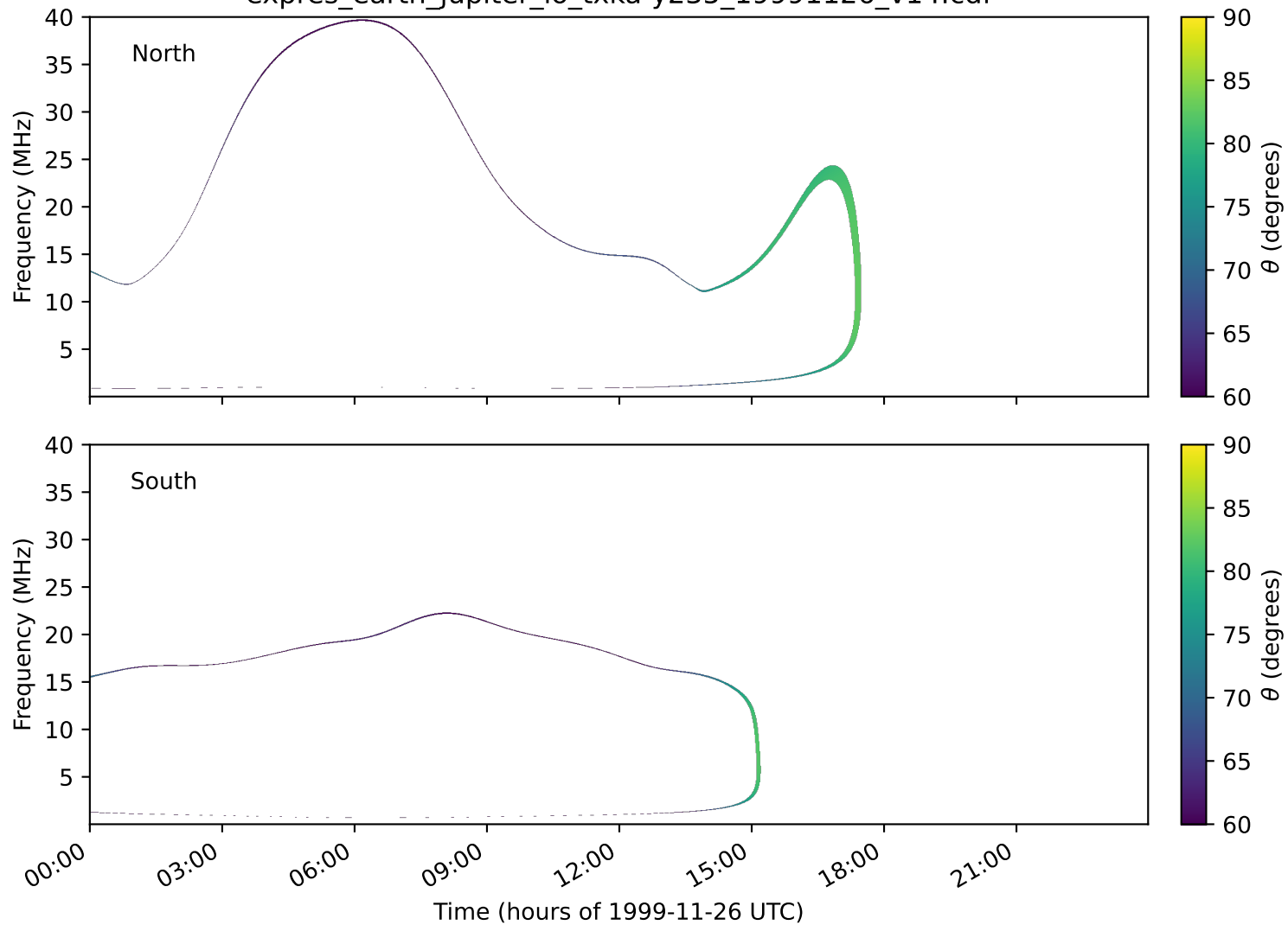
expres_earth_jupiter_io_txka-y235_19991126_v14.cdf
