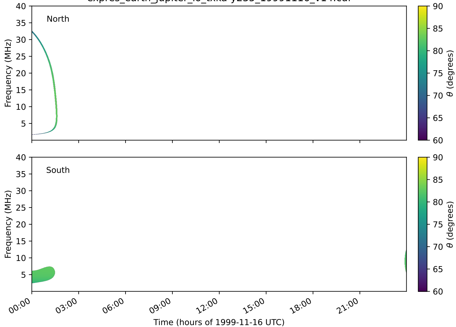
expres_earth_jupiter_io_txka-y235_19991116_v14.cdf
