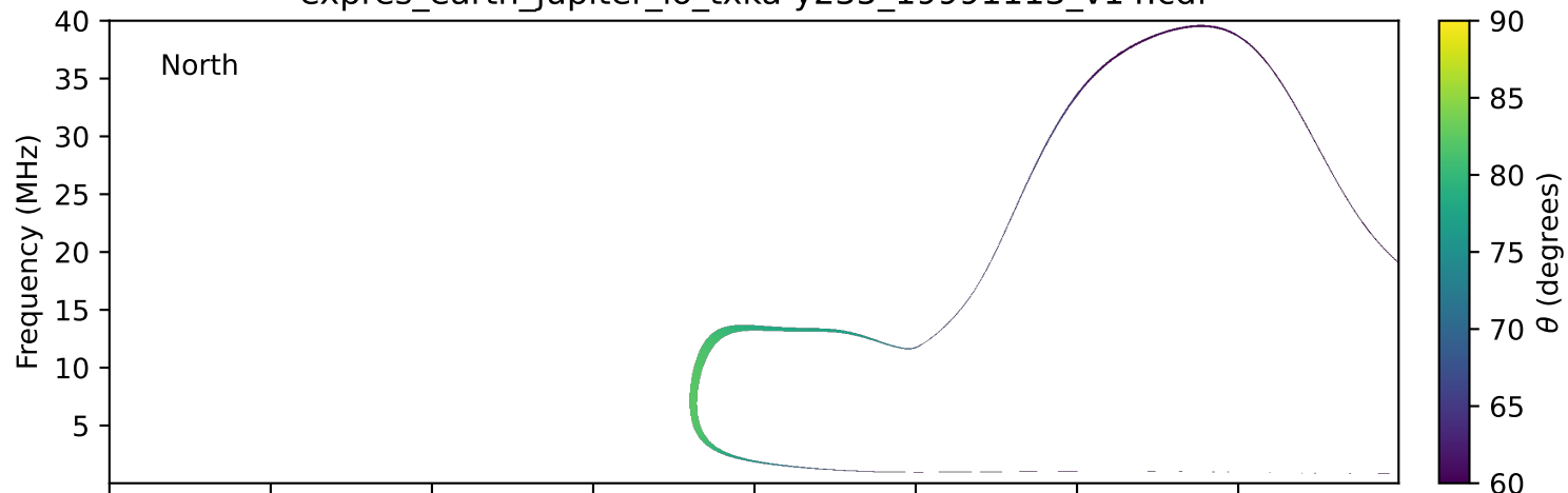
expres_earth_jupiter_io_txka-y235_19991113_v14.cdf
