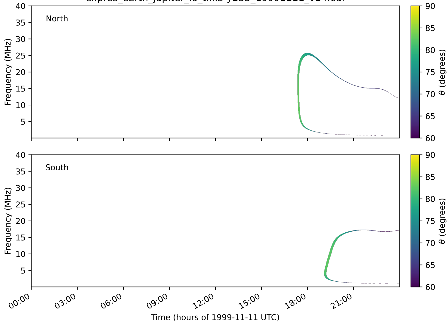
expres_earth_jupiter_io_txka-y235_19991111_v14.cdf
