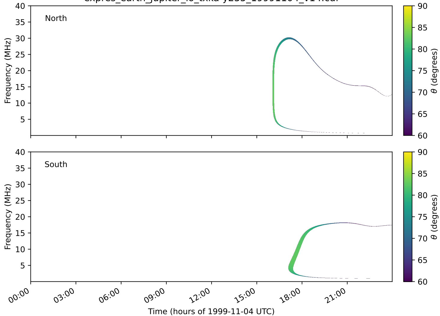
expres_earth_jupiter_io_txka-y235_19991104_v14.cdf
