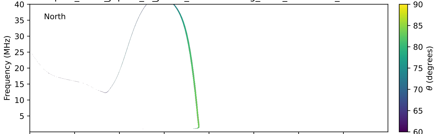
expres_earth_jupiter_io_jrm09_lossc-wid1deg_3kev_19991128_v11.cdf
