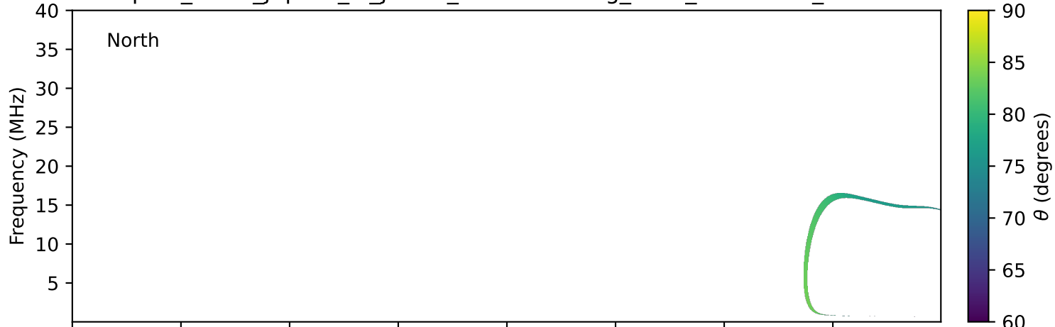
expres_earth_jupiter_io_jrm09_lossc-wid1deg_3kev_19991125_v11.cdf
