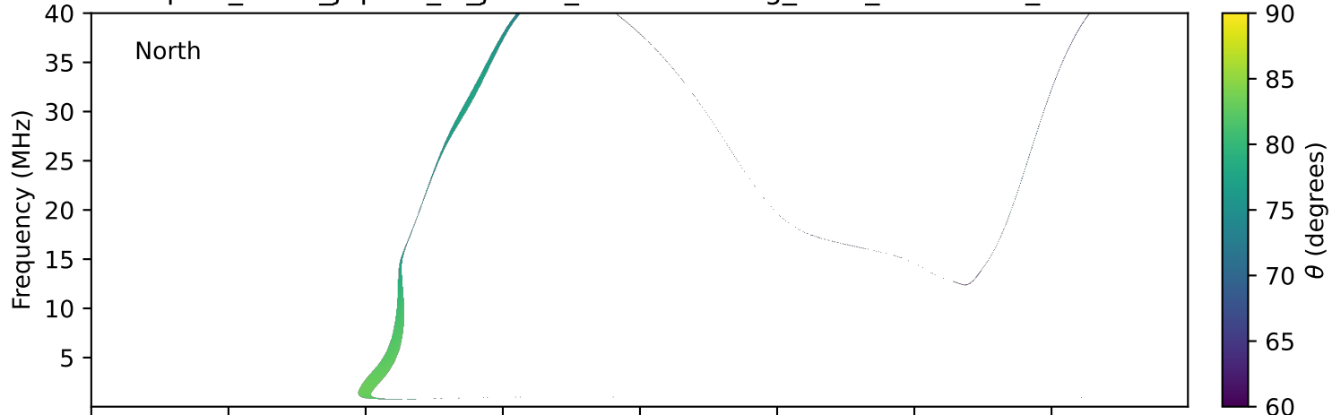
expres_earth_jupiter_io_jrm09_lossc-wid1deg_3kev_19991115_v11.cdf
