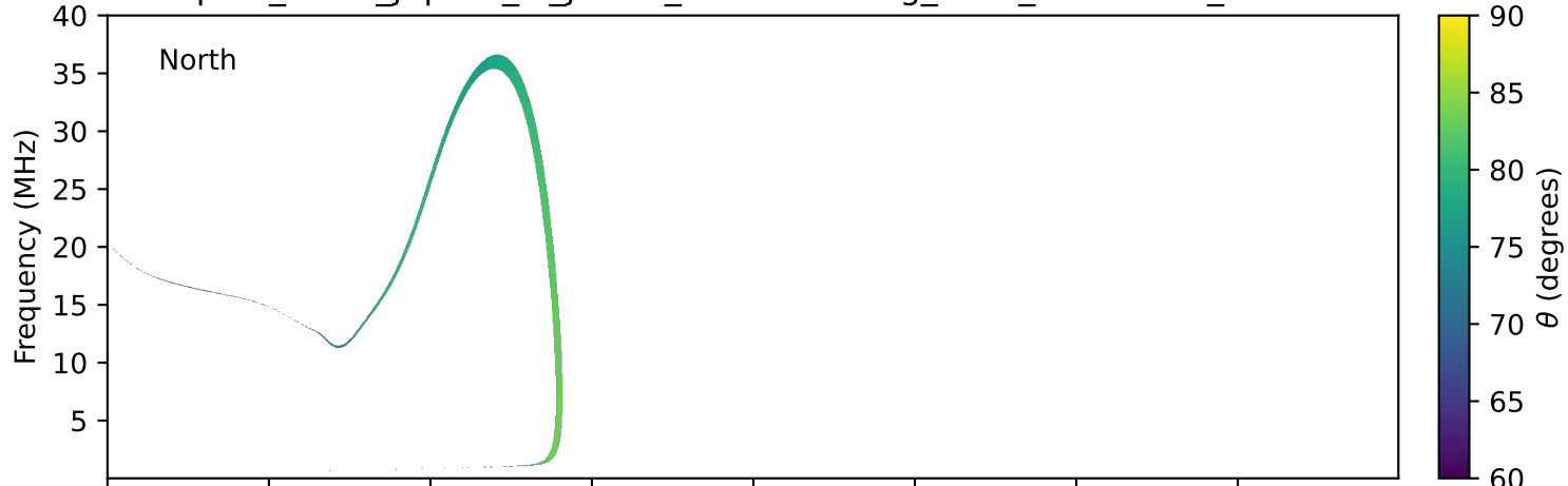
expres_earth_jupiter_io_jrm09_lossc-wid1deg_3kev_19991114_v11.cdf
