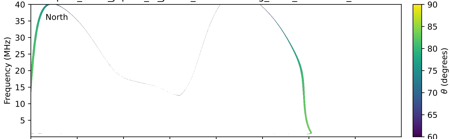
expres_earth_jupiter_io_jrm09_lossc-wid1deg_3kev_19991110_v11.cdf
