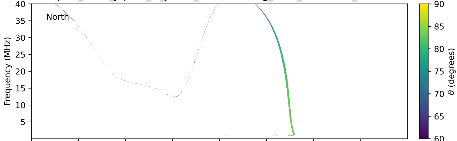
expres_earth_jupiter_io_jrm09_lossc-wid1deg_3kev_19991103_v11.cdf
