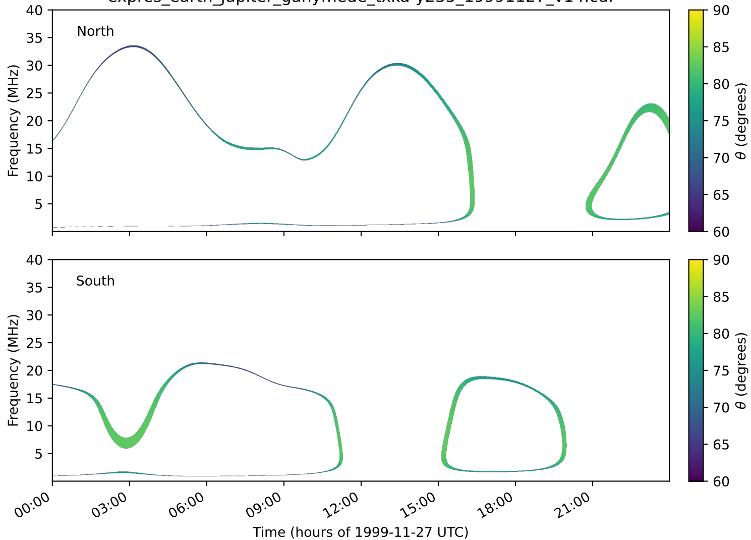
expres_earth_jupiter_ganymede_txka-y235_19991127_v14.cdf
