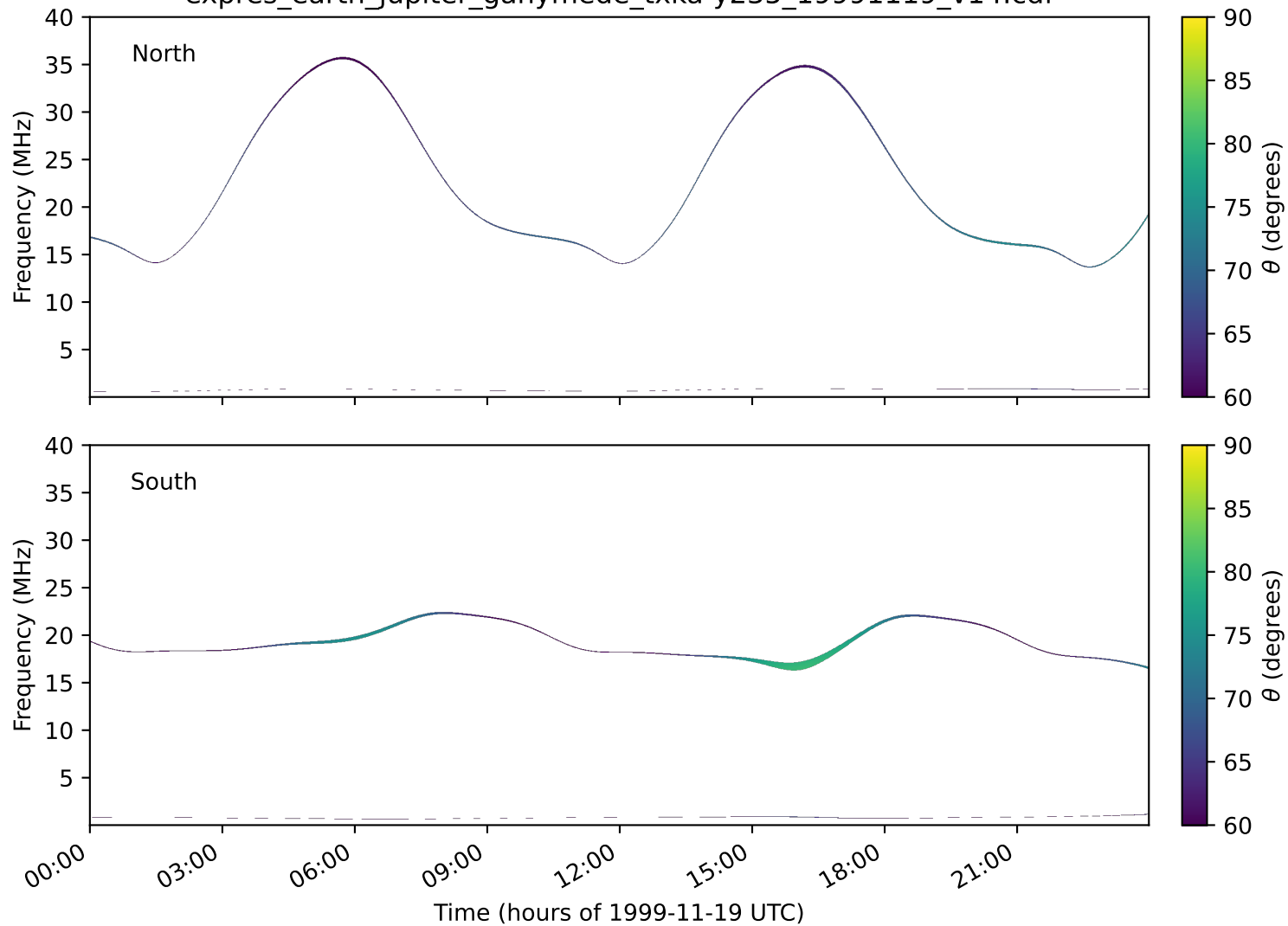
expres_earth_jupiter_ganymede_txka-y235_19991119_v14.cdf
