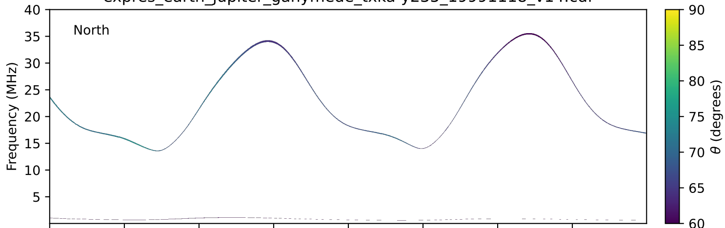
expres_earth_jupiter_ganymede_txka-y235_19991118_v14.cdf
