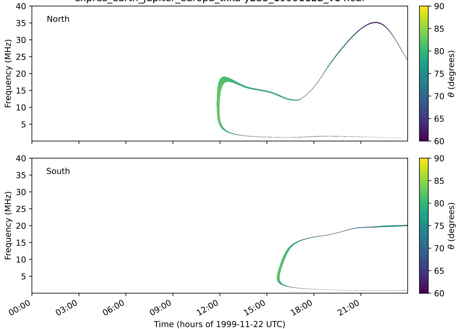
expres_earth_jupiter_europa_txka-y235_19991122_v14.cdf
