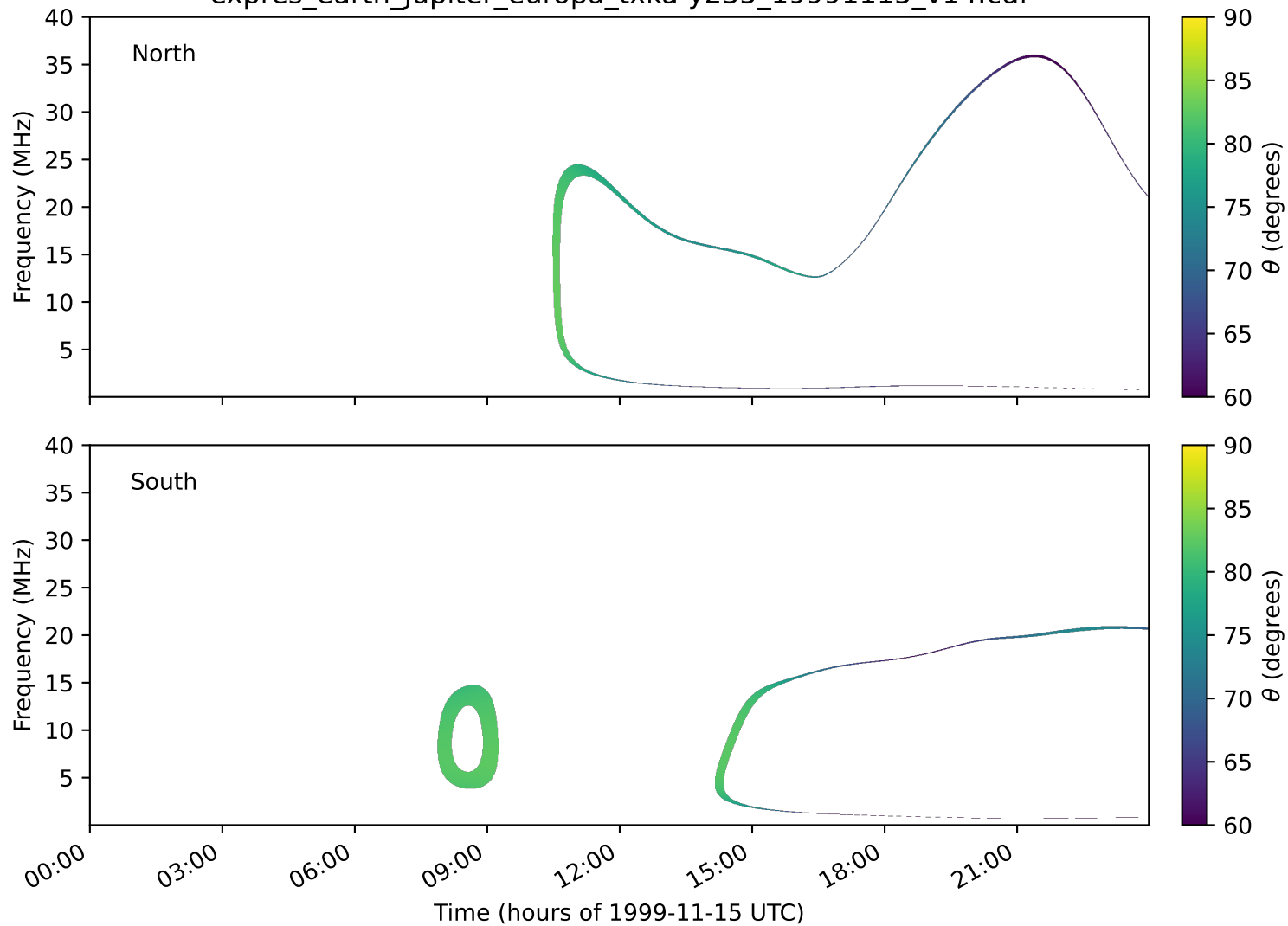
expres_earth_jupiter_europa_txka-y235_19991115_v14.cdf
