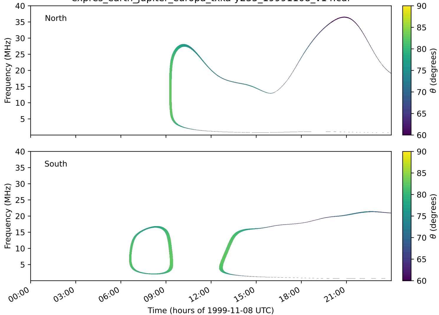
expres_earth_jupiter_europa_txka-y235_19991108_v14.cdf
