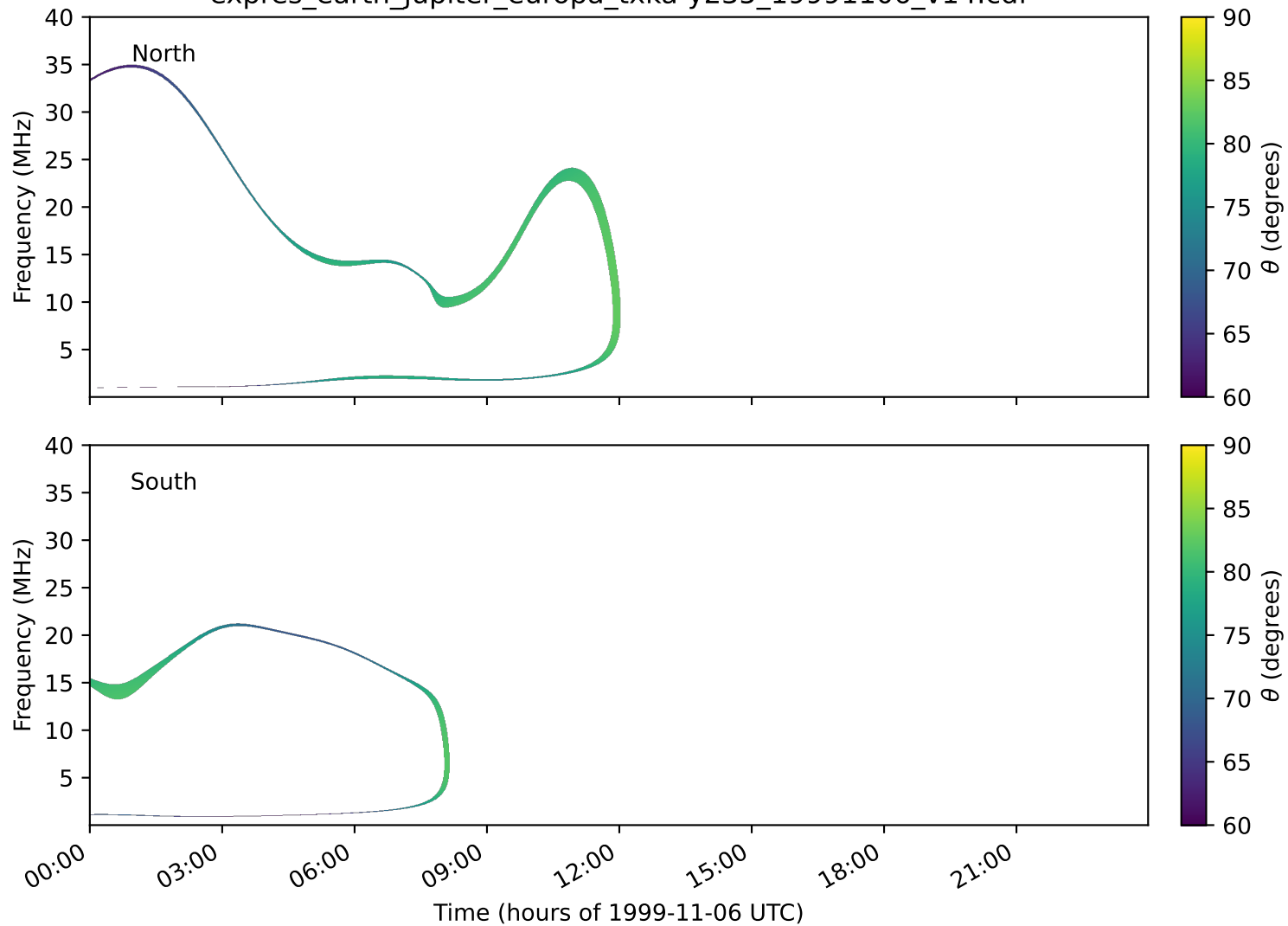
expres_earth_jupiter_europa_txka-y235_19991106_v14.cdf
