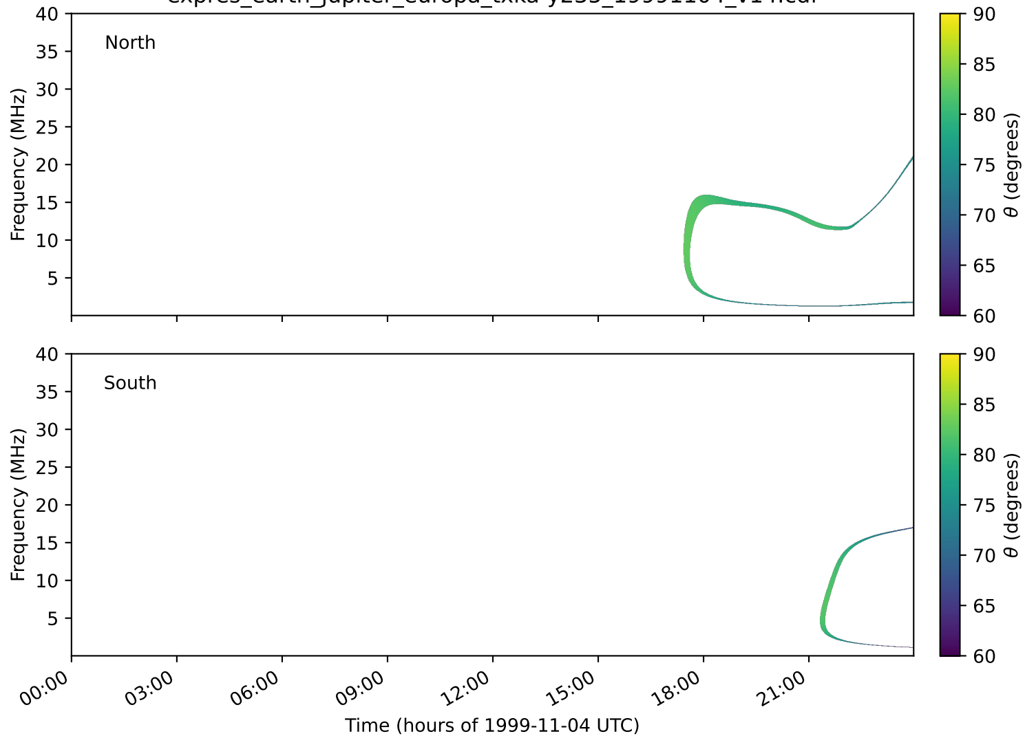
expres_earth_jupiter_europa_txka-y235_19991104_v14.cdf
