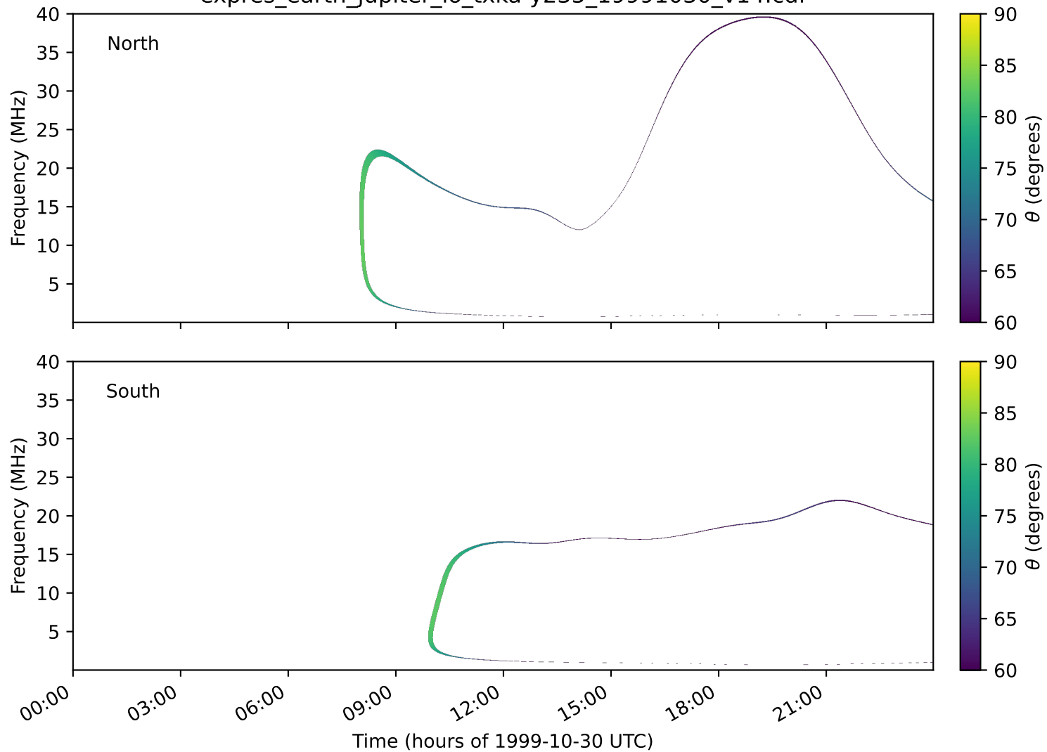
expres_earth_jupiter_io_txka-y235_19991030_v14.cdf
