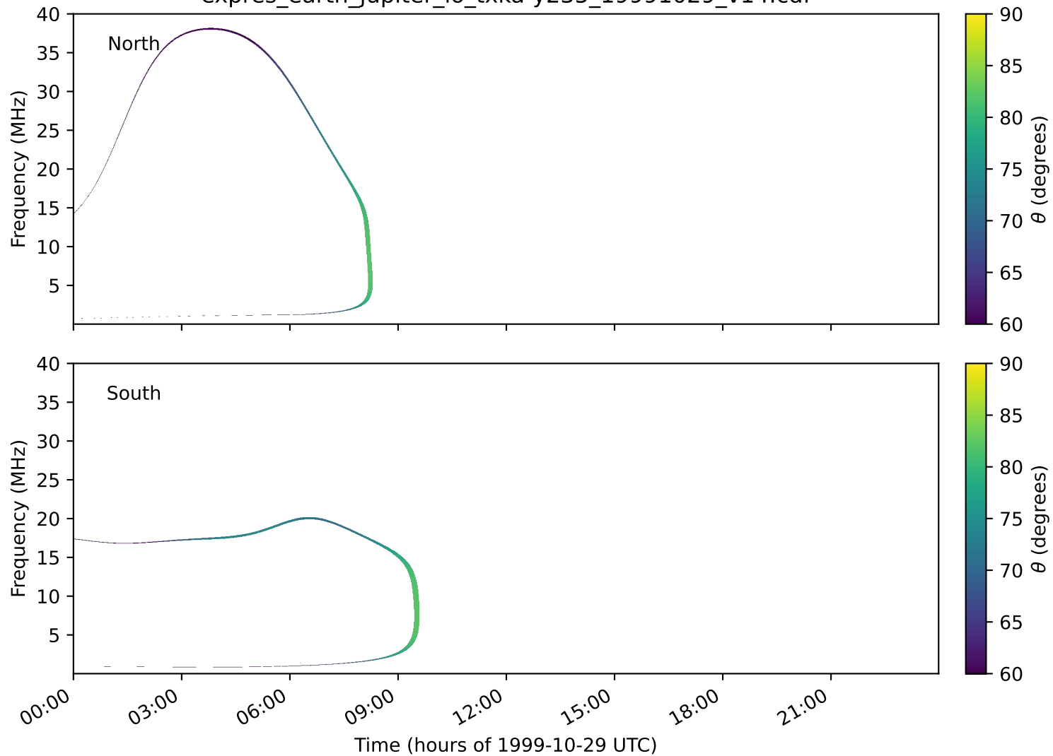
expres_earth_jupiter_io_txka-y235_19991029_v14.cdf
