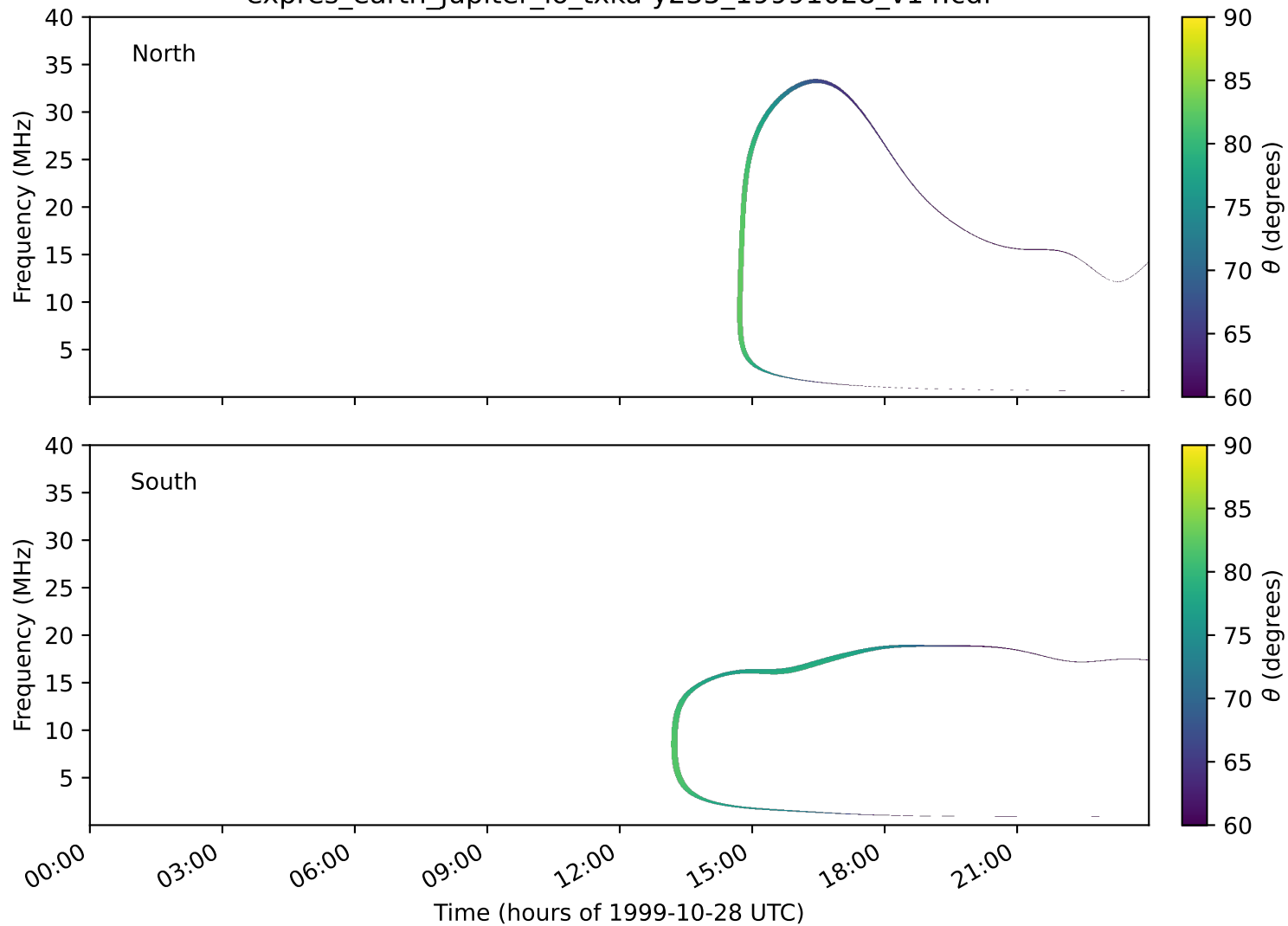
expres_earth_jupiter_io_txka-y235_19991028_v14.cdf
