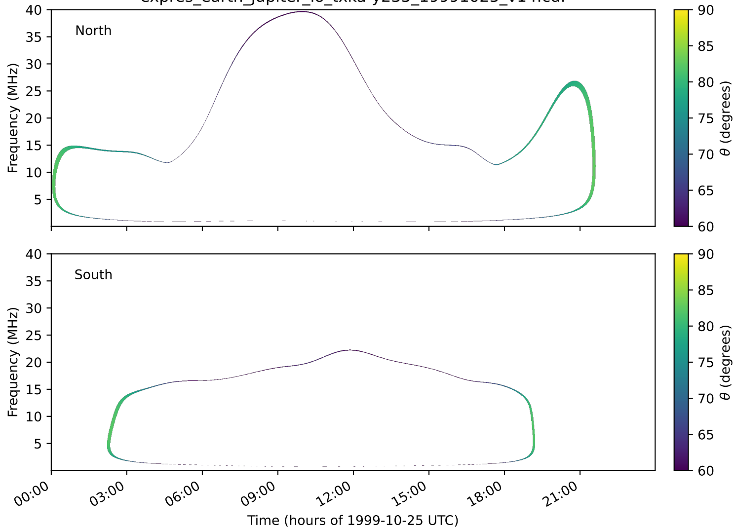
expres_earth_jupiter_io_txka-y235_19991025_v14.cdf
