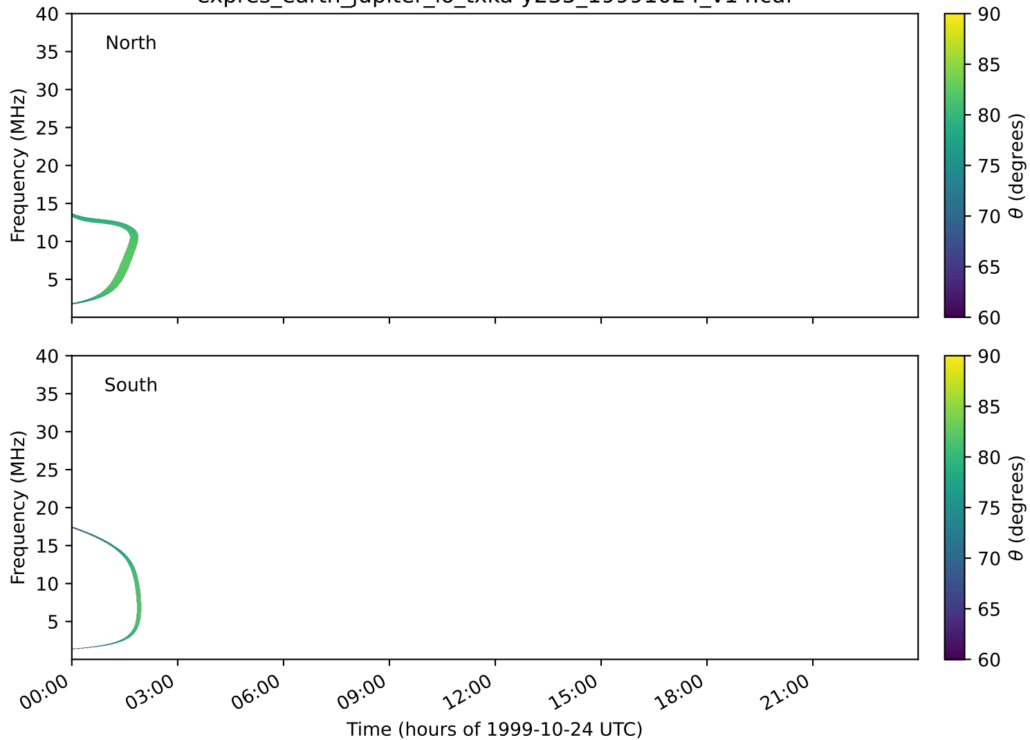
expres_earth_jupiter_io_txka-y235_19991024_v14.cdf
