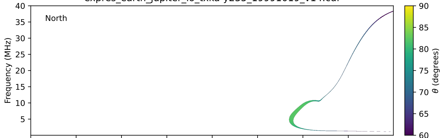
expres_earth_jupiter_io_txka-y235_19991019_v14.cdf
