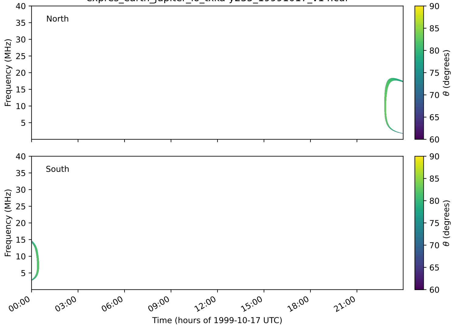
expres_earth_jupiter_io_txka-y235_19991017_v14.cdf
