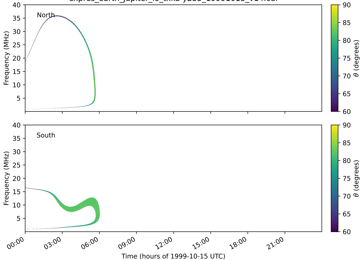
expres_earth_jupiter_io_txka-y235_19991015_v14.cdf
