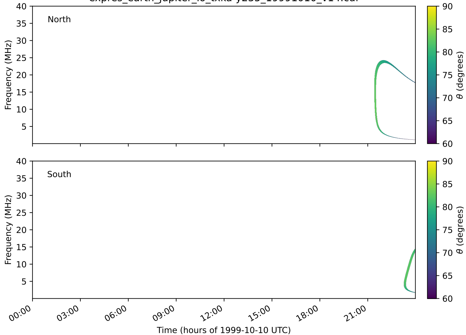
expres_earth_jupiter_io_txka-y235_19991010_v14.cdf
