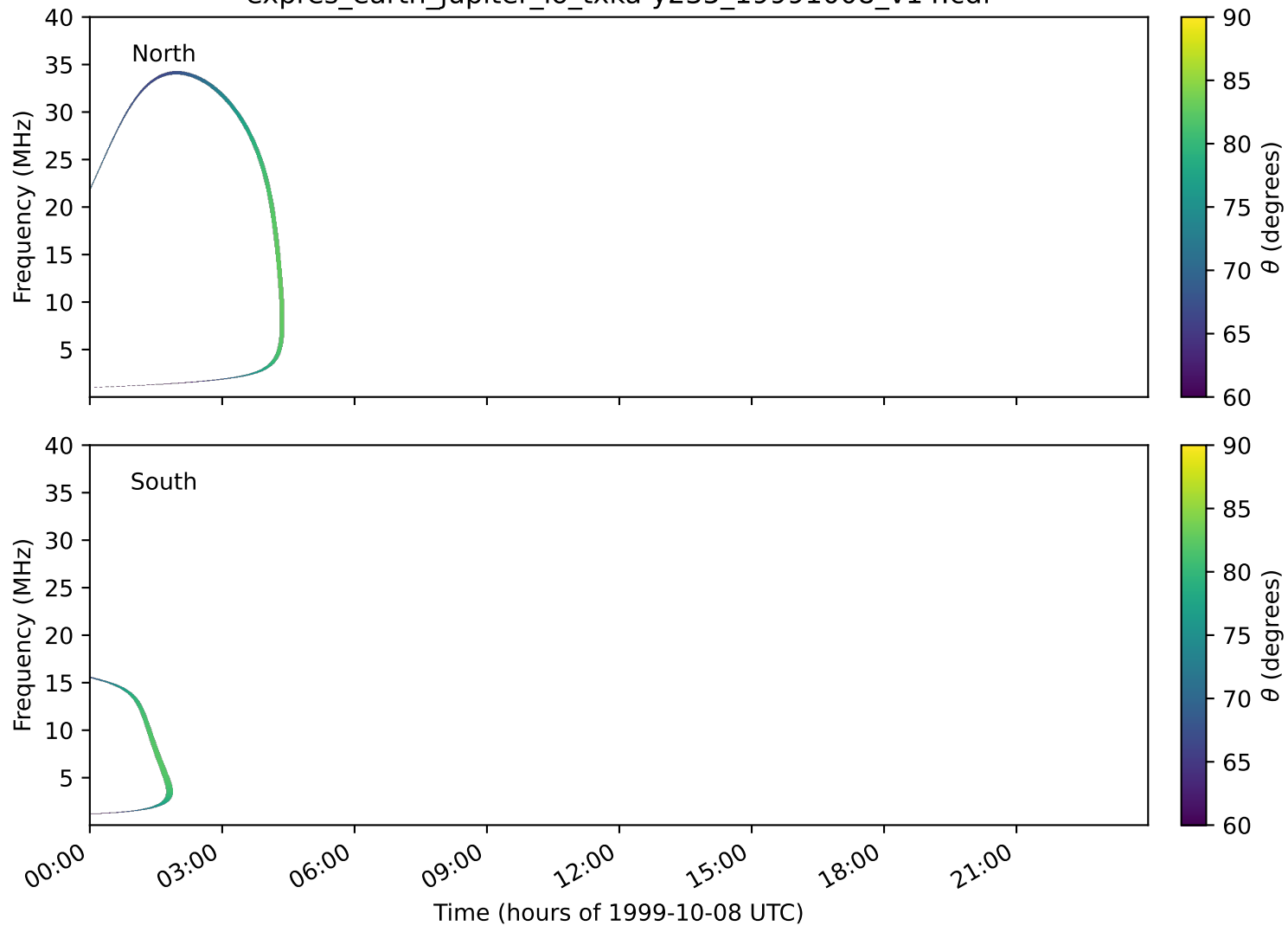
expres_earth_jupiter_io_txka-y235_19991008_v14.cdf
