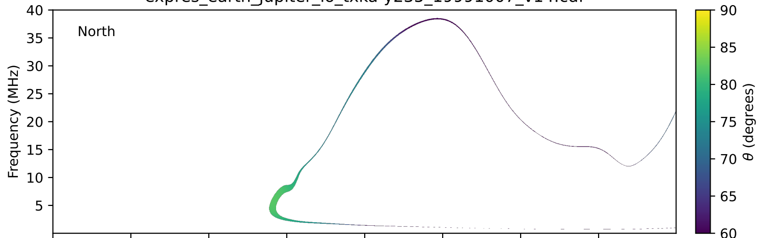
expres_earth_jupiter_io_txka-y235_19991007_v14.cdf
