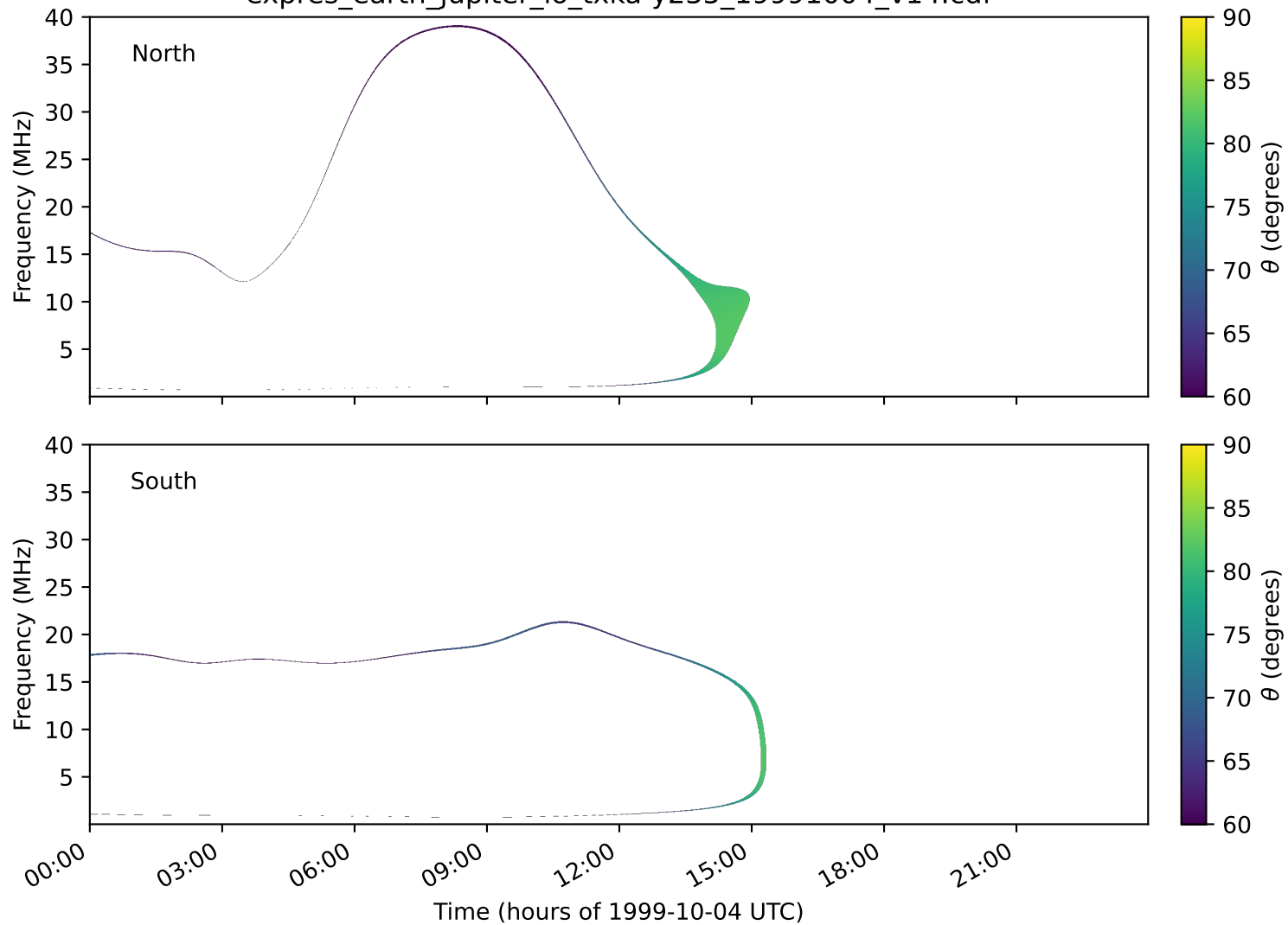
expres_earth_jupiter_io_txka-y235_19991004_v14.cdf
