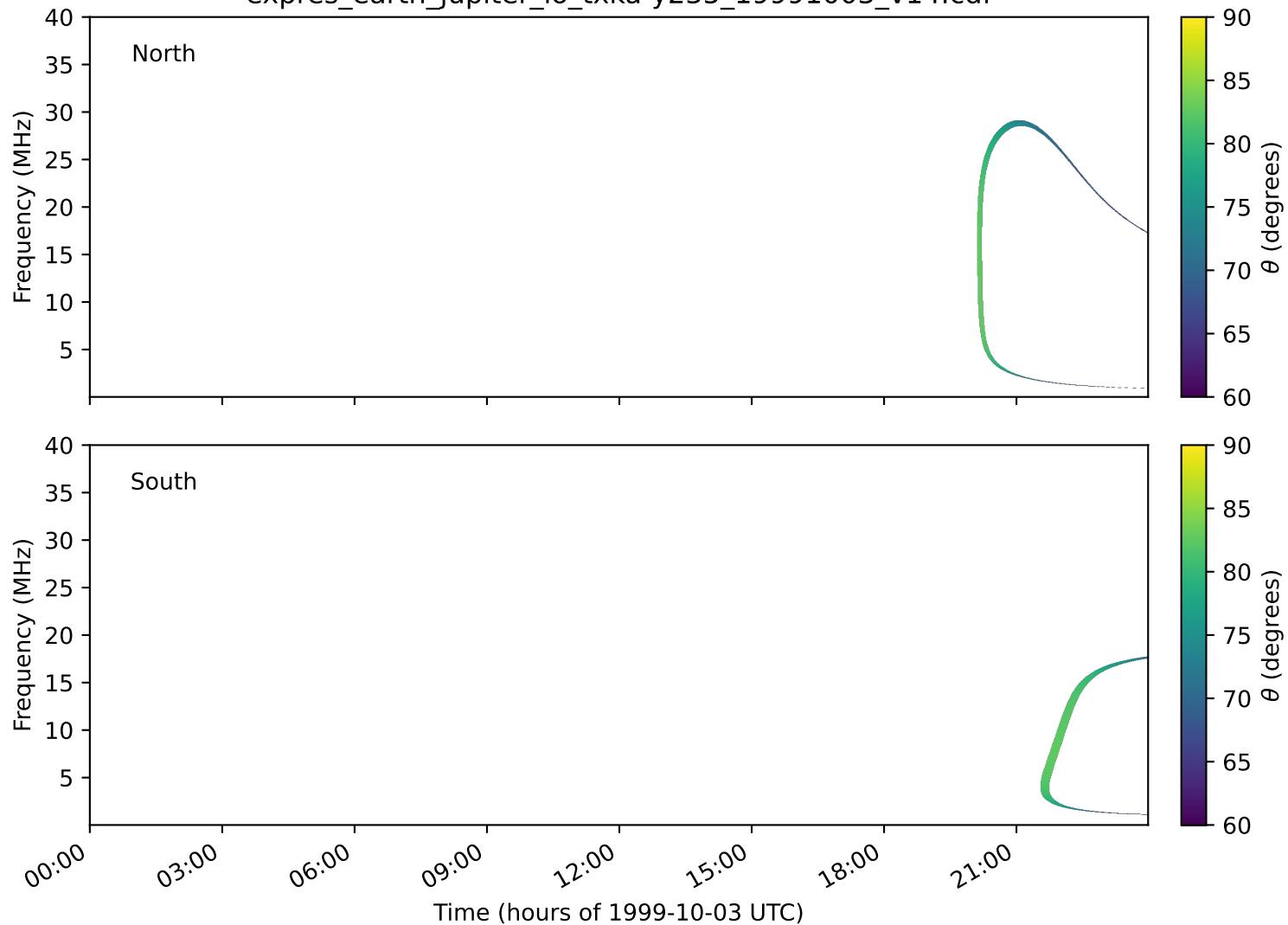
expres_earth_jupiter_io_txka-y235_19991003_v14.cdf
