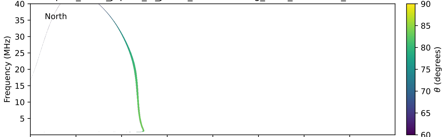
expres_earth_jupiter_io_jrm09_lossc-wid1deg_3kev_19991022_v11.cdf
