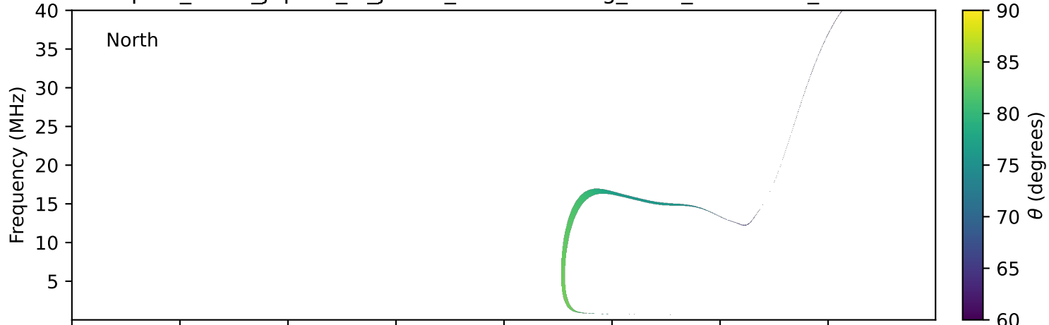
expres_earth_jupiter_io_jrm09_lossc-wid1deg_3kev_19991005_v11.cdf
