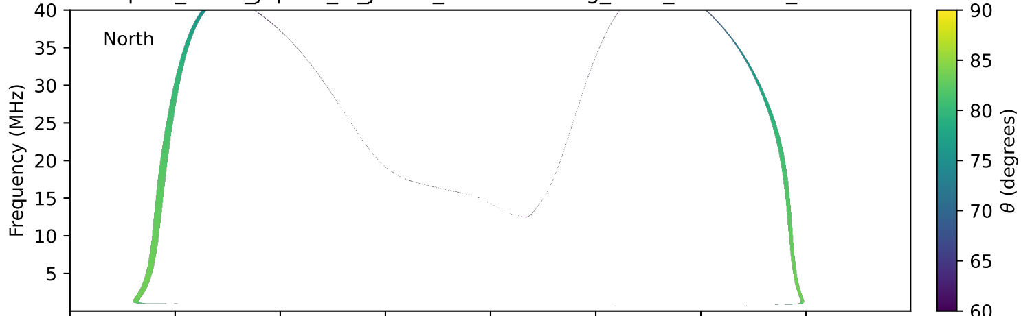
expres_earth_jupiter_io_jrm09_lossc-wid1deg_3kev_19991002_v11.cdf
