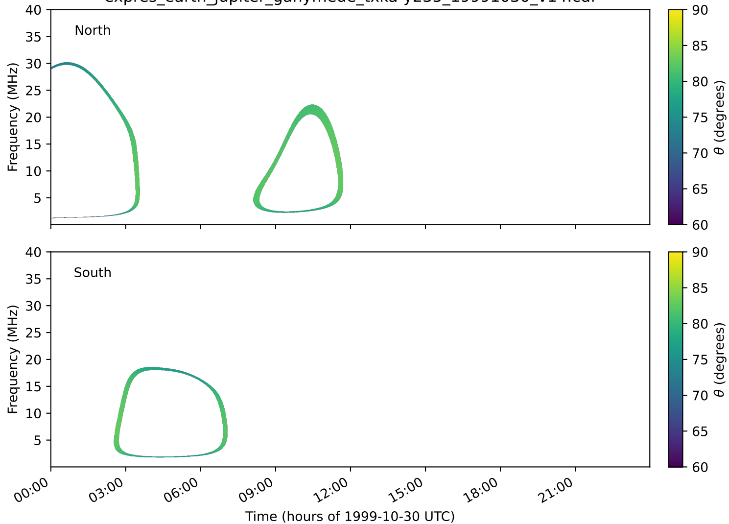
expres_earth_jupiter_ganymede_txka-y235_19991030_v14.cdf
