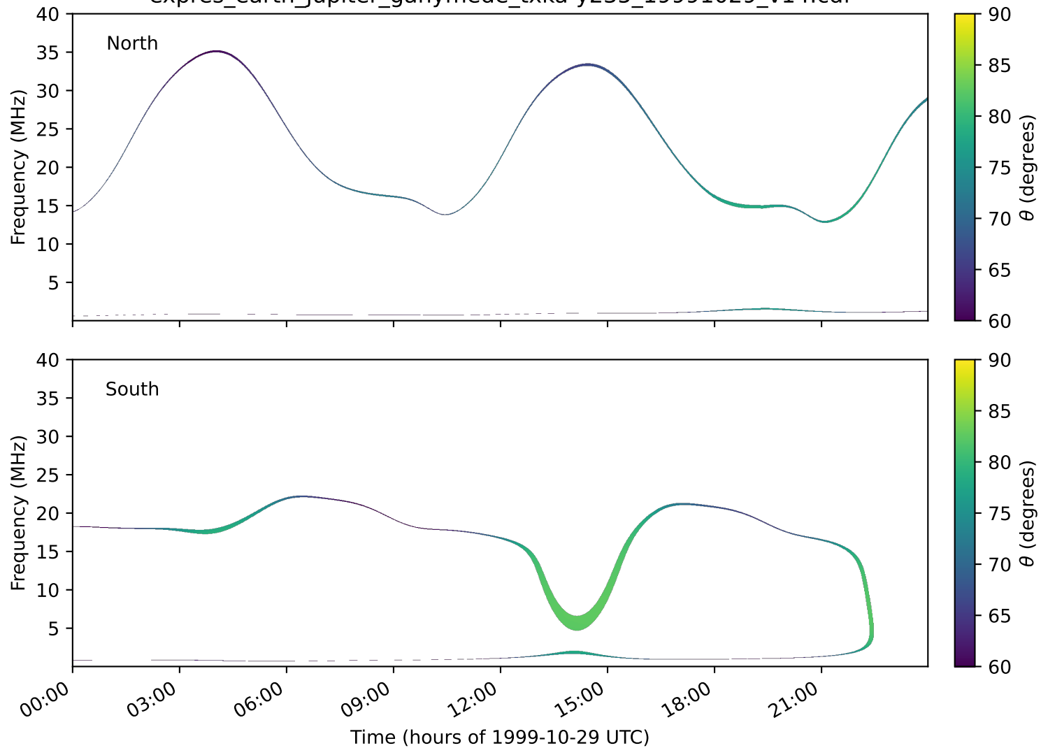
expres_earth_jupiter_ganymede_txka-y235_19991029_v14.cdf
