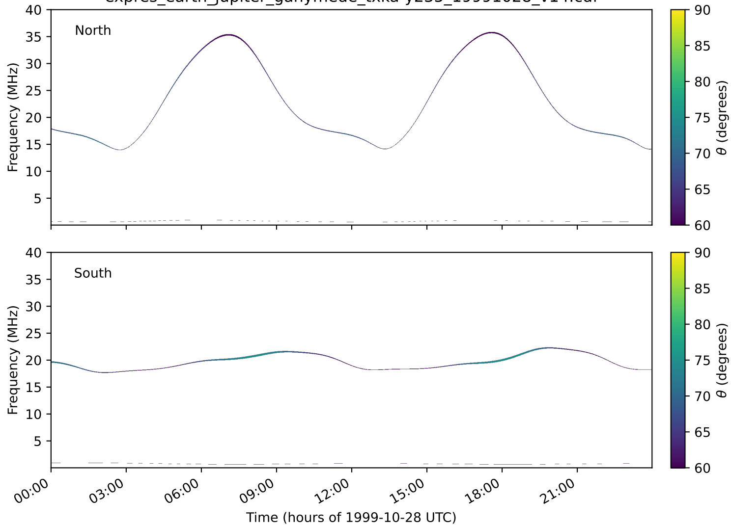
expres_earth_jupiter_ganymede_txka-y235_19991028_v14.cdf
