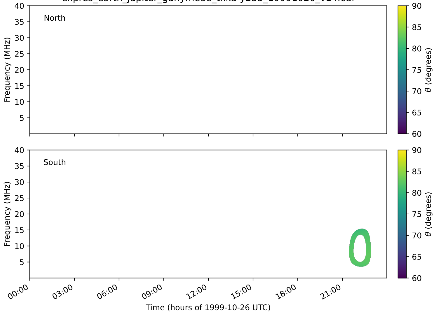
expres_earth_jupiter_ganymede_txka-y235_19991026_v14.cdf
