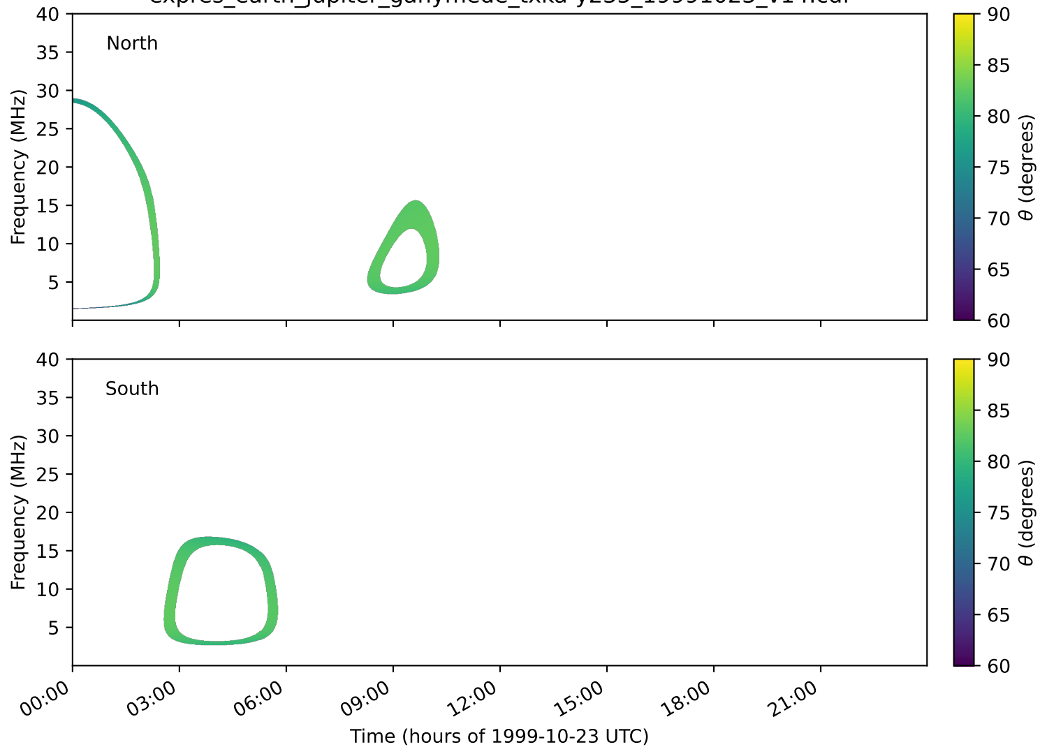
expres_earth_jupiter_ganymede_txka-y235_19991023_v14.cdf
