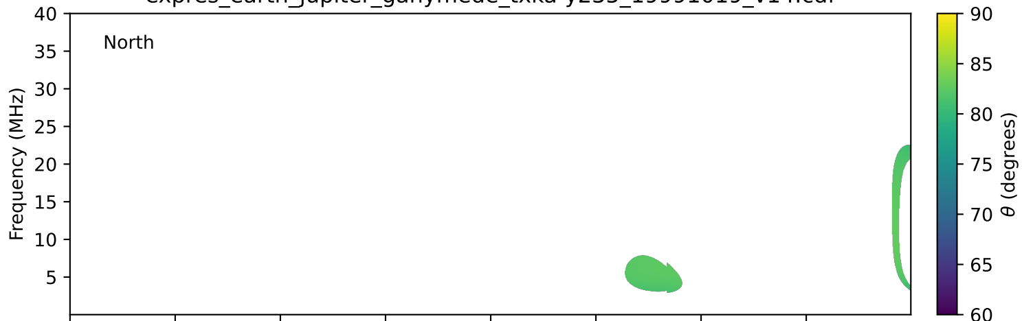
expres_earth_jupiter_ganymede_txka-y235_19991019_v14.cdf
