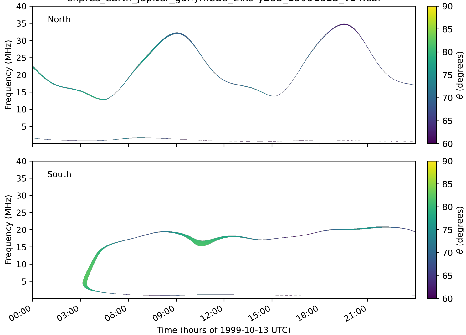
expres_earth_jupiter_ganymede_txka-y235_19991013_v14.cdf
